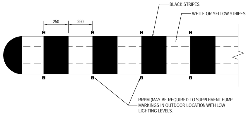
OFF ROAD ROAD HUMP MARKING SCALE : NTS
