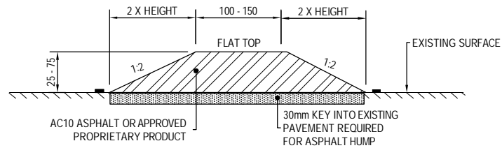
OFF ROAD ROAD HUMP SECTION SCALE : NTS
